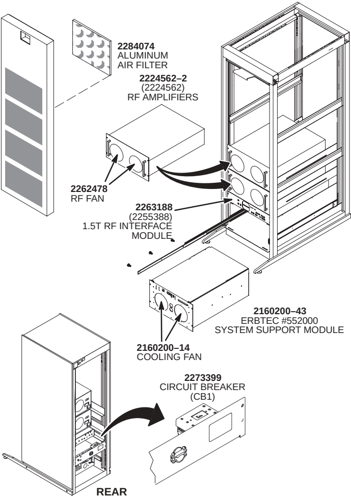
SRF CABINET
